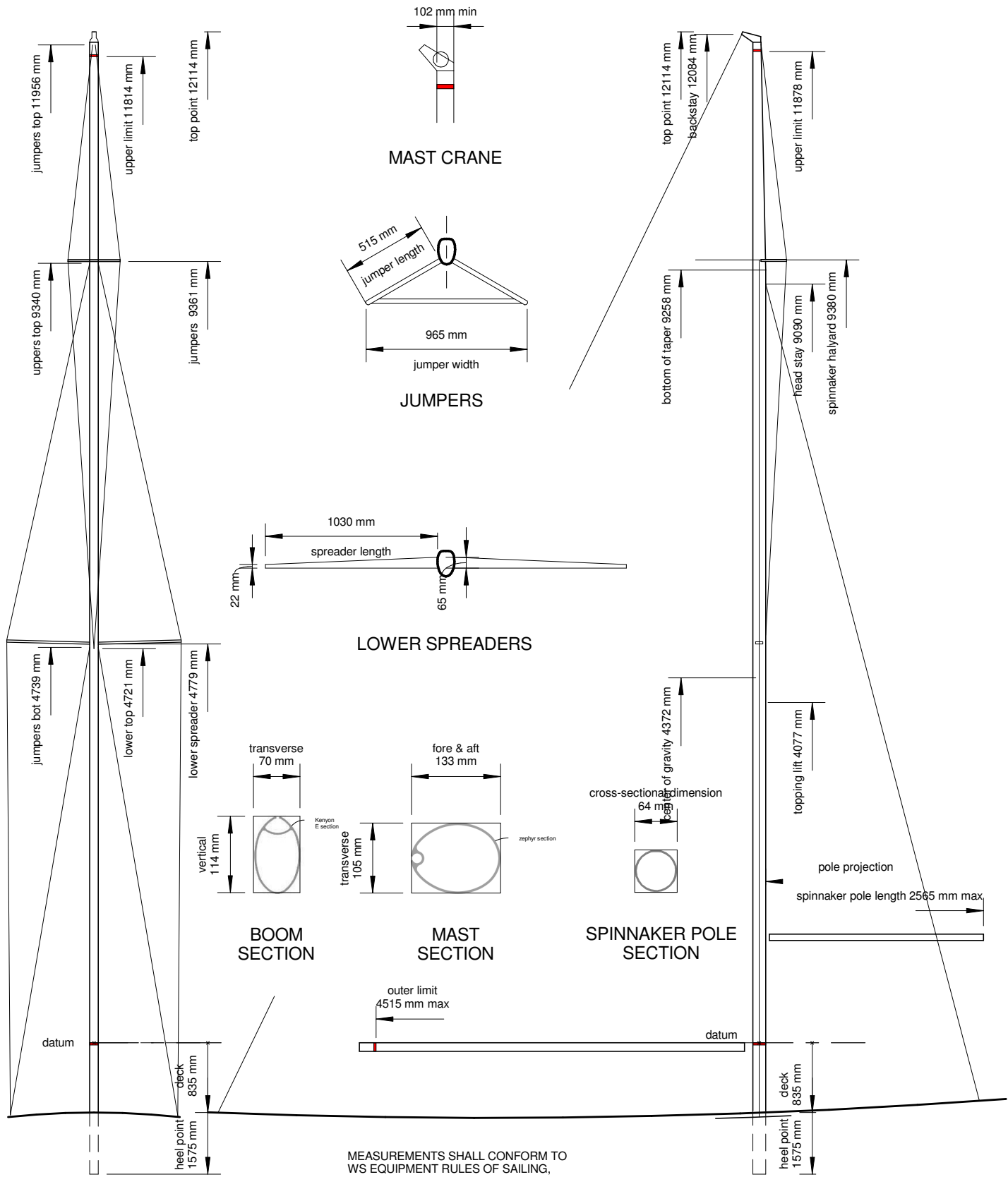
MAST SECTION
