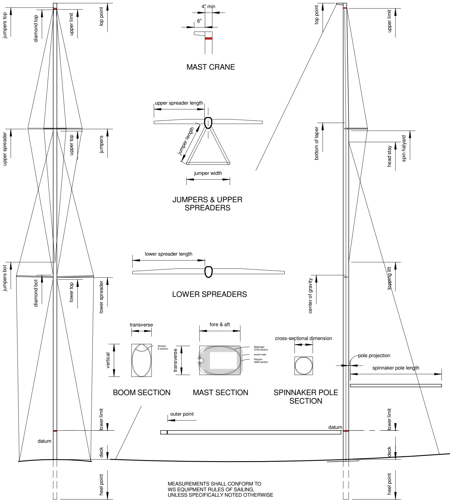
MAST SECTION
