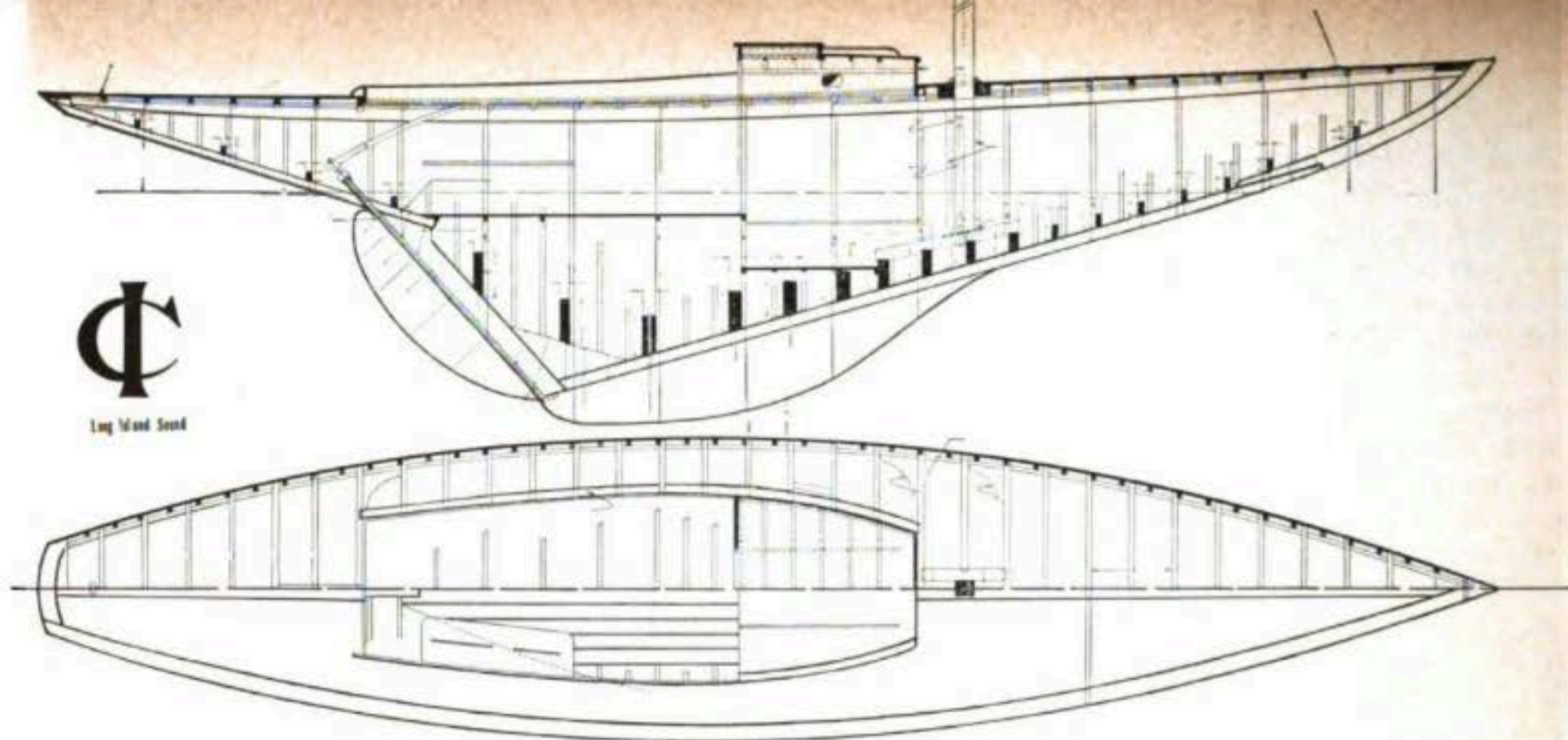
The I.O.D. is a 33-foot sloop (21'5" lwl) with a 6'9" beam and 5'4" draft. She carries 426 feet of sail on a 45-foot mast and, in the words of Uffa Fox, has lines "as clean as a smelt's."
